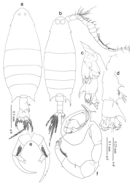
Figure 4. Labidocera kroeyeri (Brady, 1883). Female, a, whole animal, dorsal view; c, Pdg5 and urosome, lateral view; d, urosome, dorsal view; e, fifth legs. Male, b, whole animal, dorsal view; f, fifth legs.
